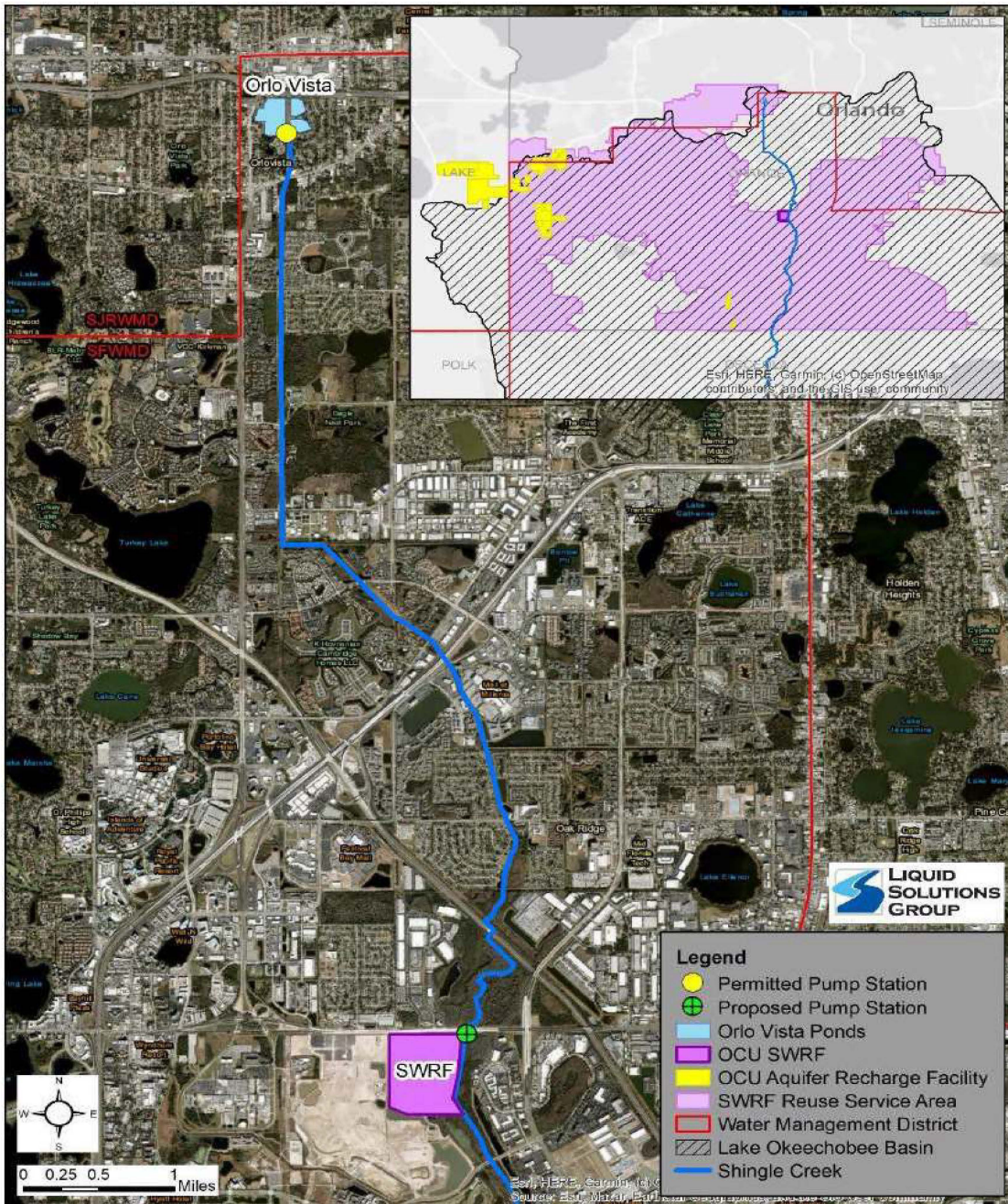
Figure 1: Site Plan
