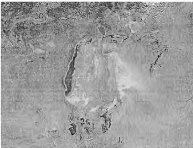
Aral Sea dust storm, March 2010
