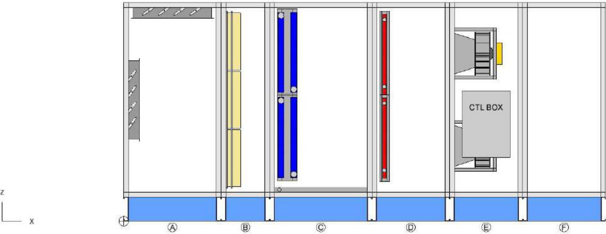
RIGHT ELEVATION VIEW
