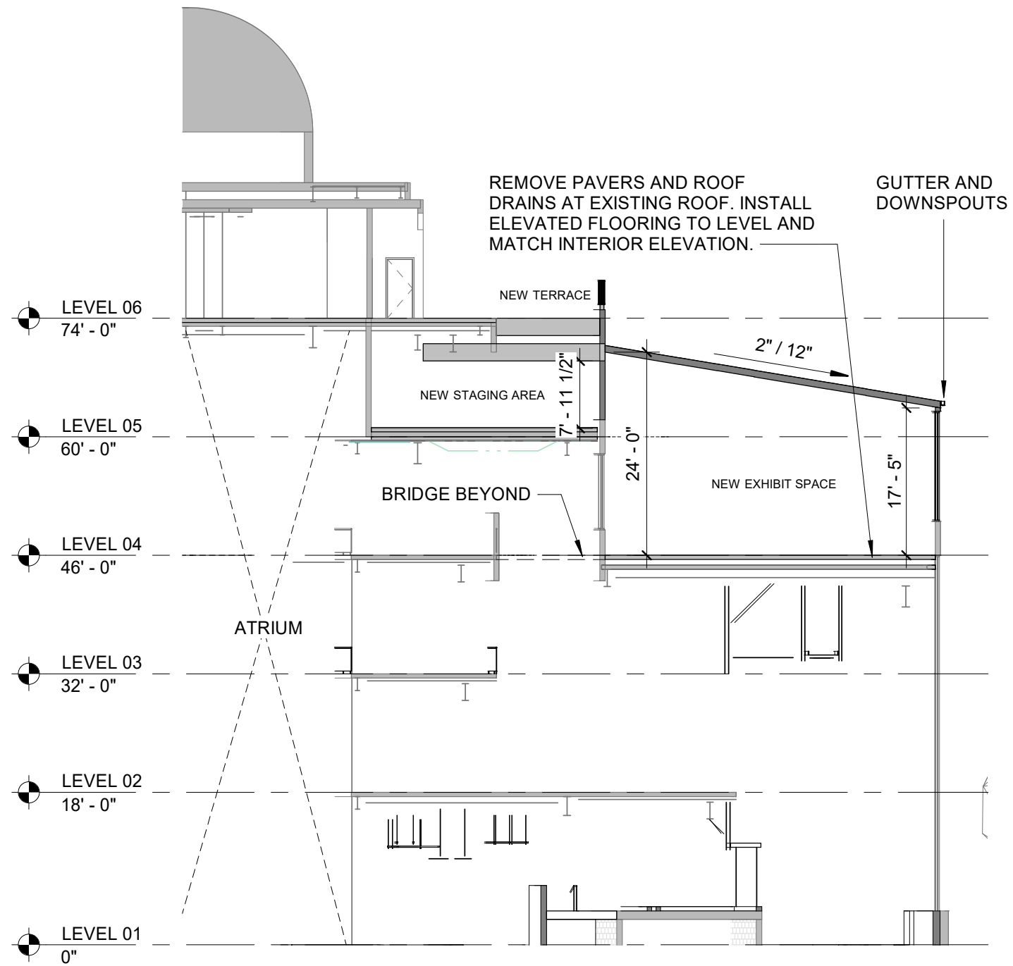
SECTION OPTION 2
