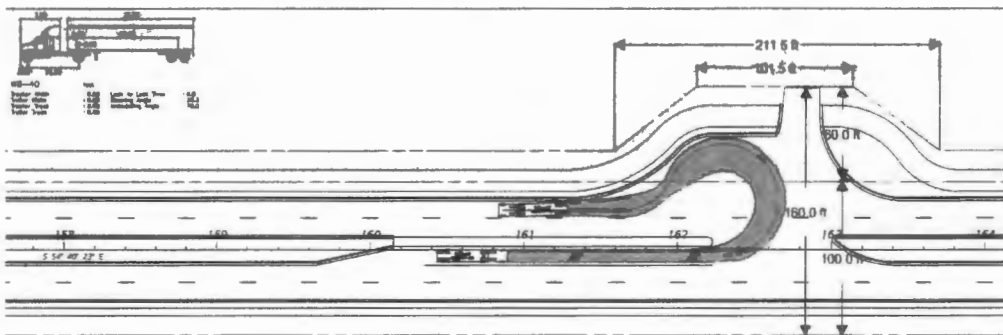
Figure 6-1: Typical U-turn Layout
