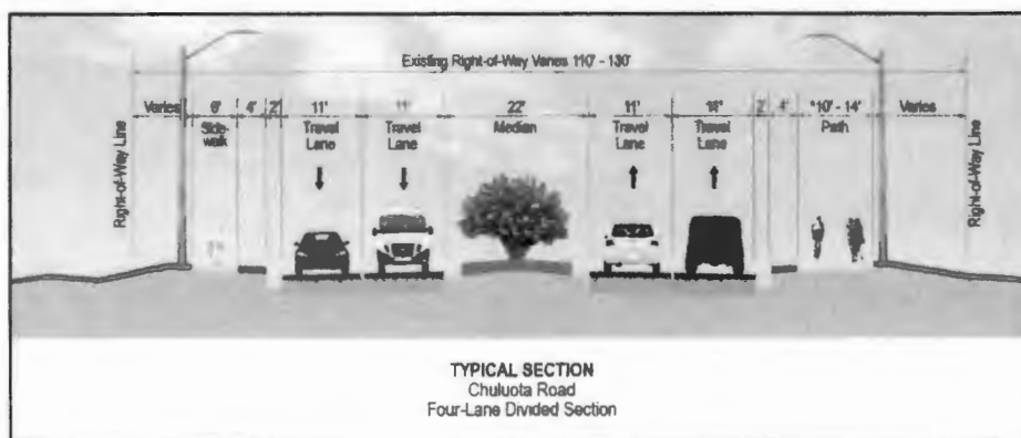
Figure 6-2 Proposed Typical Section
