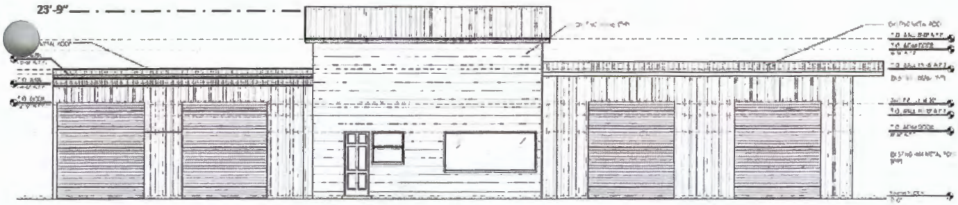
Front Elevation – West
