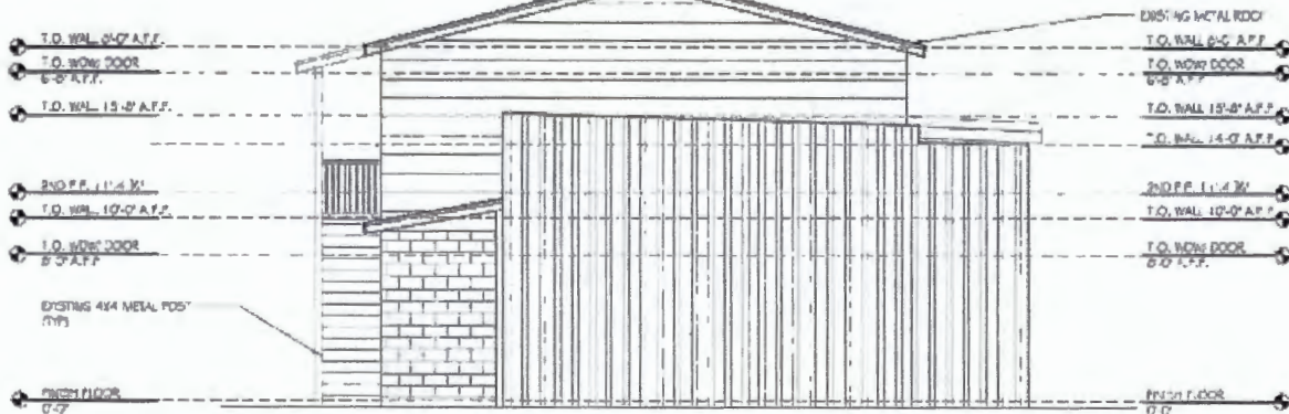
Left Elevation – North
