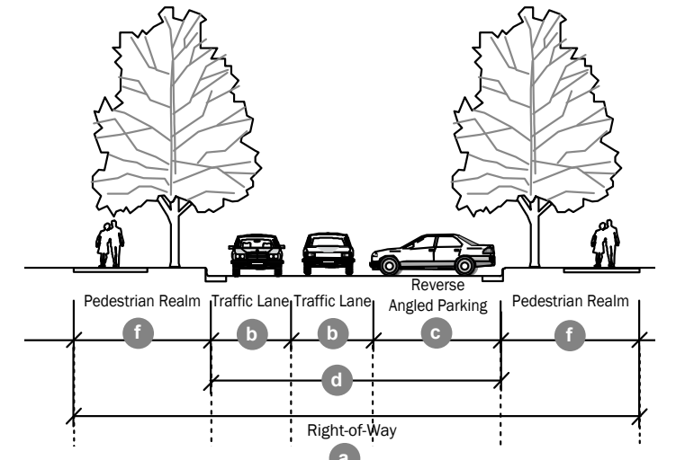
Figure (16). Alternative Local Street
