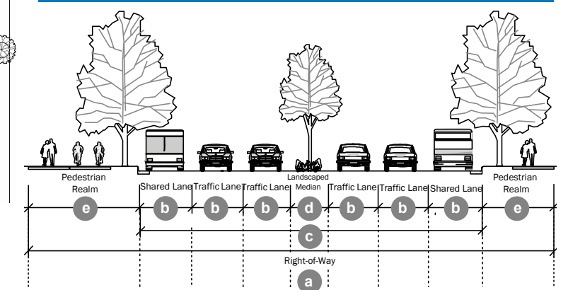
Figure (22). Alternative Six Lane Boulevard.
