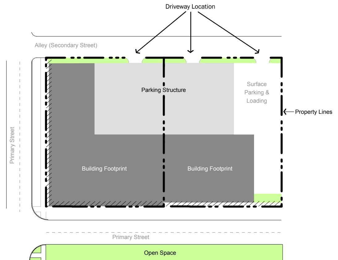
Figure (45). Driveway Location.
