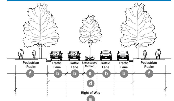
Figure (20). Alternative Boulevard
