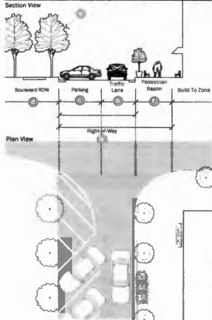
Figure (13). Typical Frontage Road
