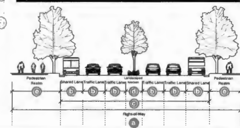
Figure (22). Alternative Six Lane Boulevard.
