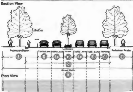
Figure (19). Typical Boulevard
