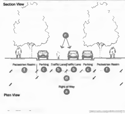
Figure (15). Typical Local Street
