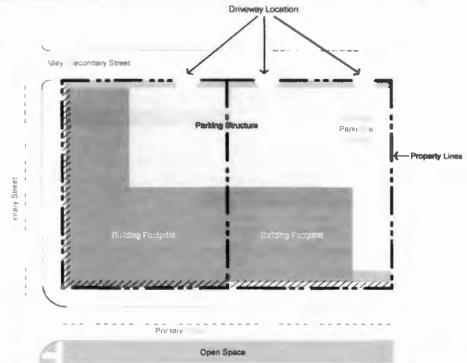
Figure (45). Driveway Location.
