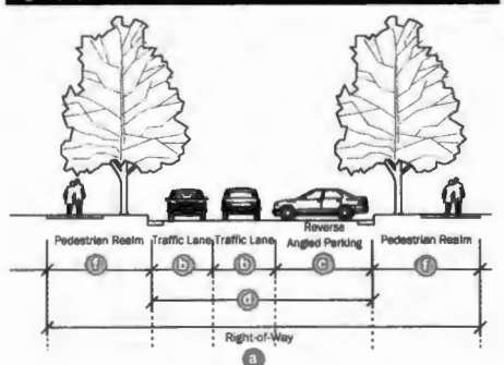
Figure (16). Alternative Local Street
