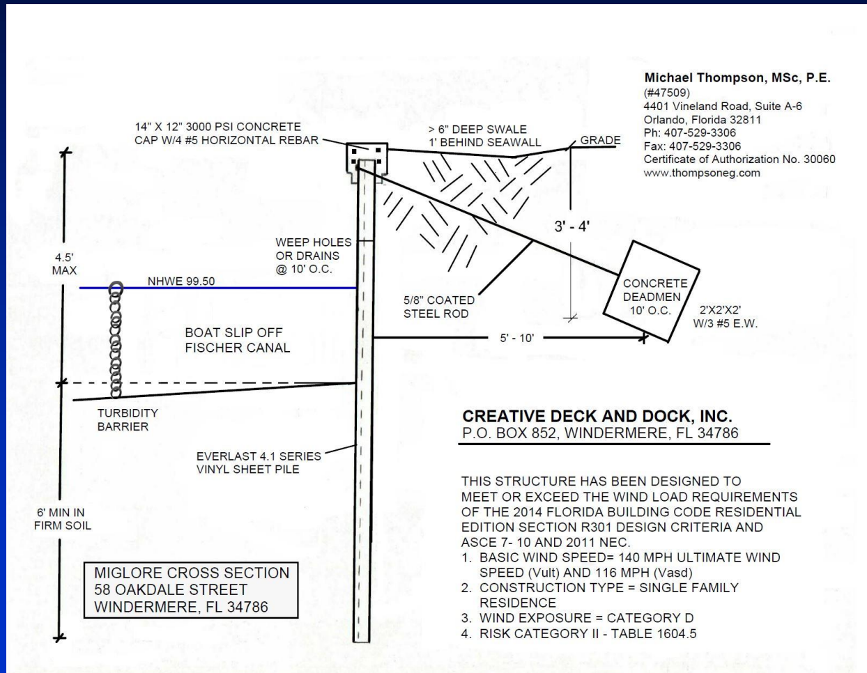
Cross-Section at Sea Wall
